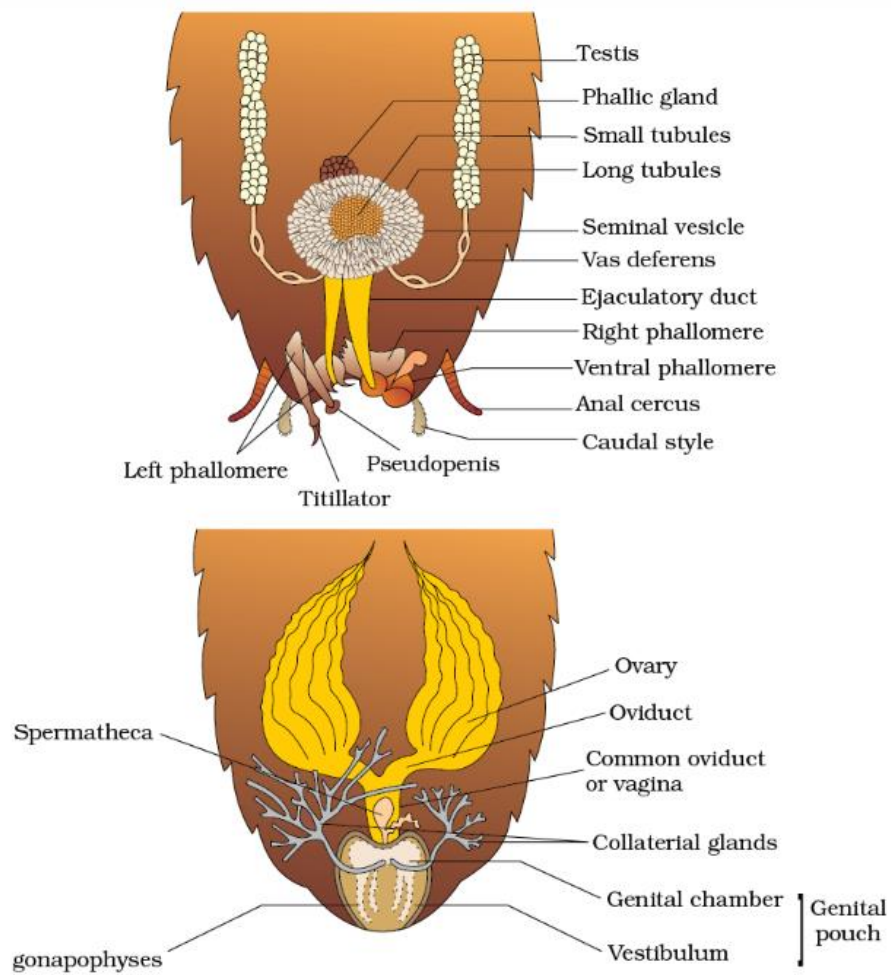
Reproductive system of cockroach: (a) male (b) female
