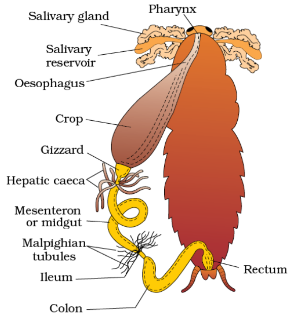
Alimentary canal of cockroach
