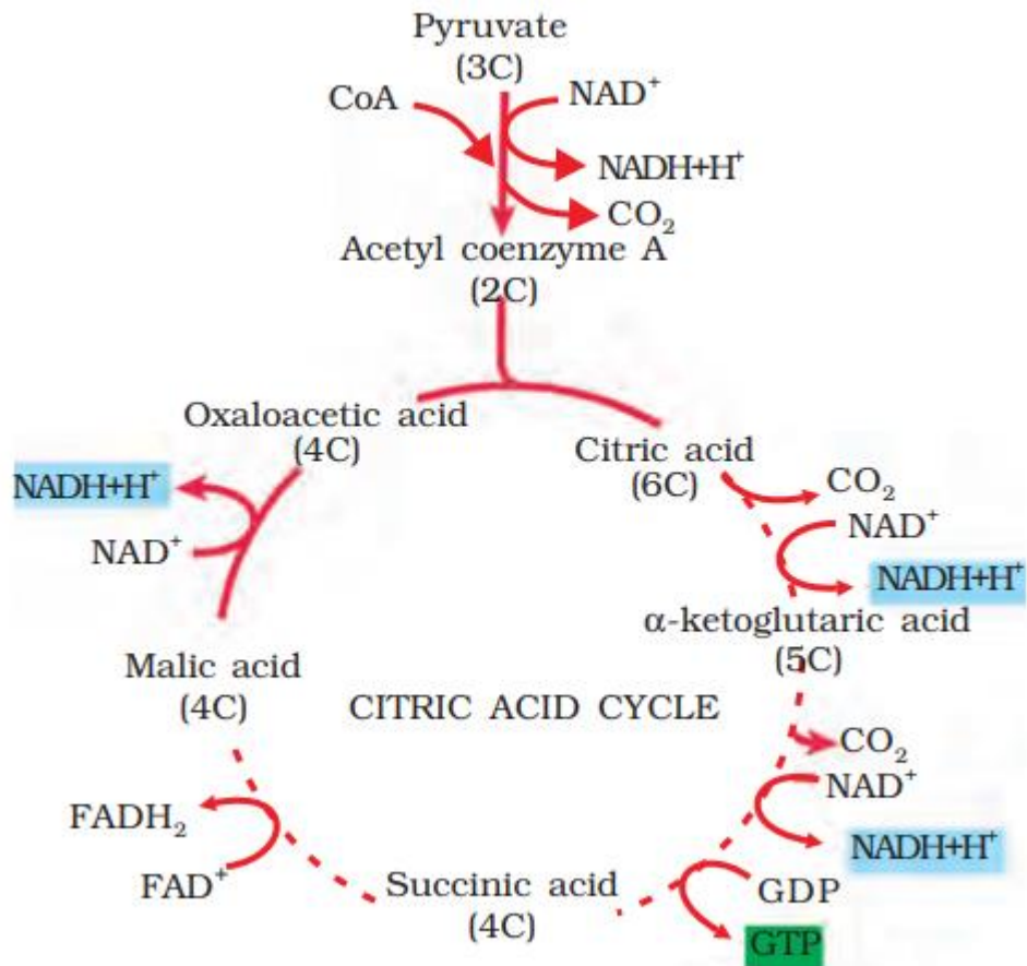
Citric acid cycle
