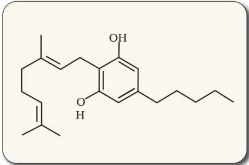
Structure of cannabinoid molecule
