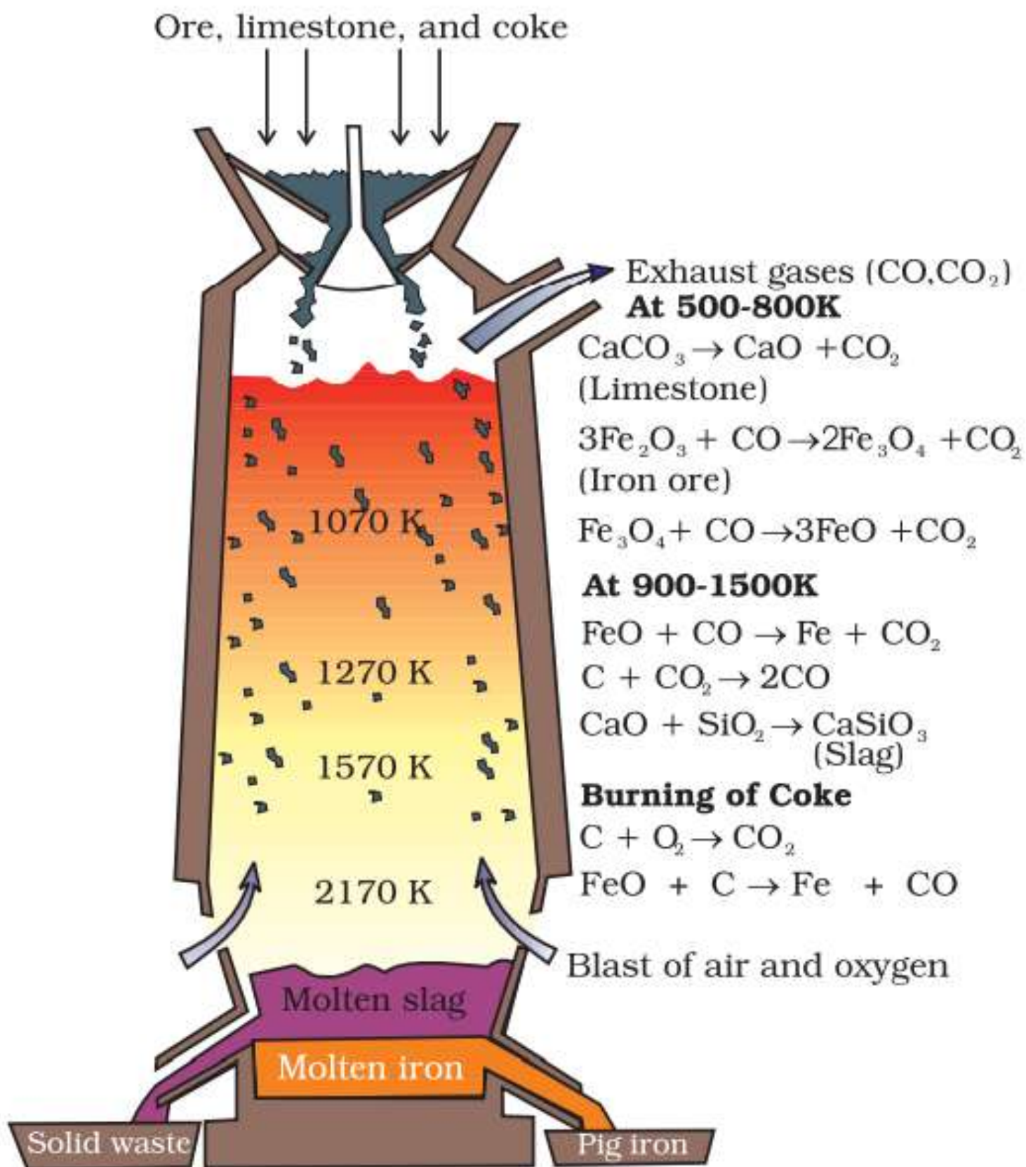
Fig. 6.5: Blast furnace
