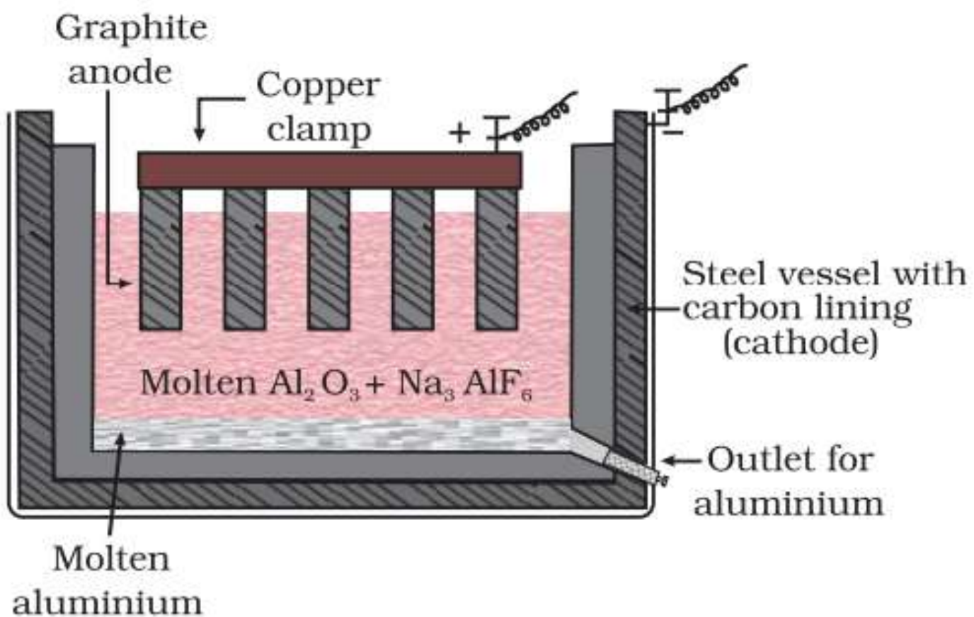
Fig. 6.6: Electrolytic cell for the extraction of aluminium
