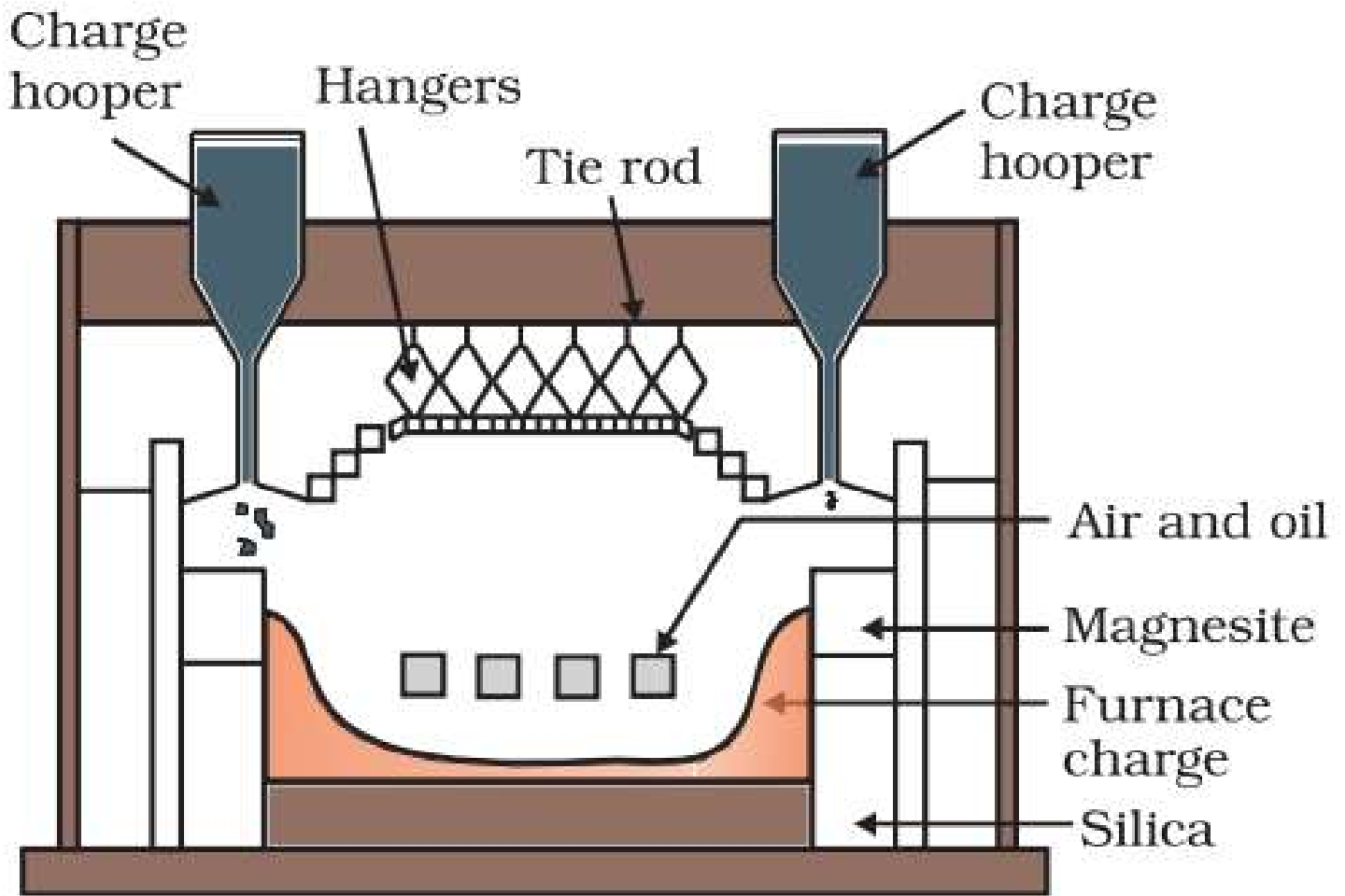
Fig. 6.3: A section of a modern reverberatory furnace
