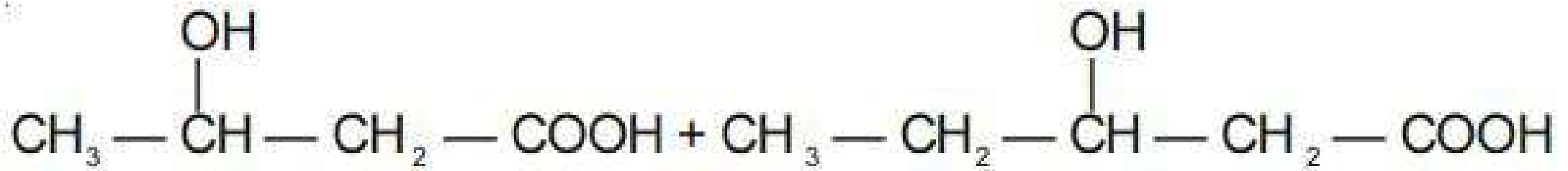
3-Hydroxybutanoic acid
