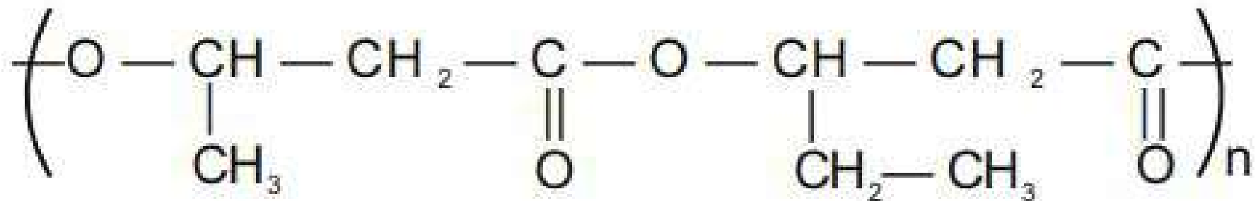
PHBV
