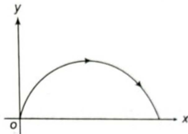
Projectile motion
