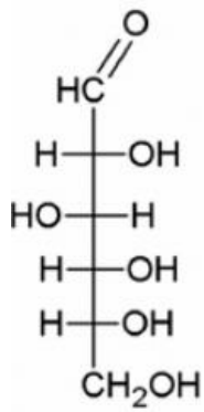
Glucose
