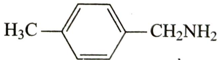
p -methyl benzylamine (1°-amine)
