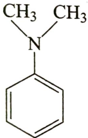
N,N-dimethylaniline (3°-amine)
