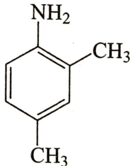
2,4-dimethylaniline (1°-amine)
