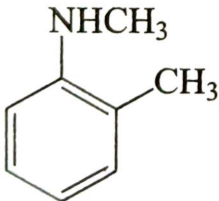
N-methyl- o -methylaniline (2°-amine)
