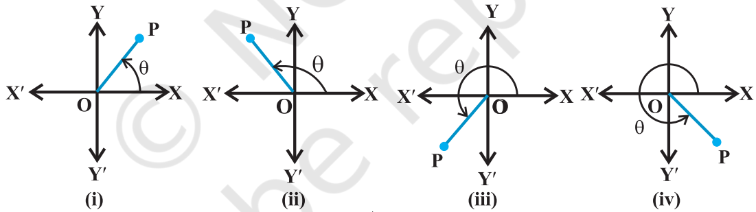
Fig 5.5 ( 0 \leq \theta < 2\pi )
