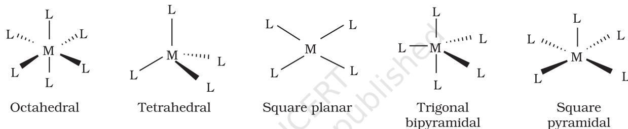
Fig. 9.1: Shapes of different coordination polyhedra. M represents the central atom/ion and L, a unidentate ligand.
